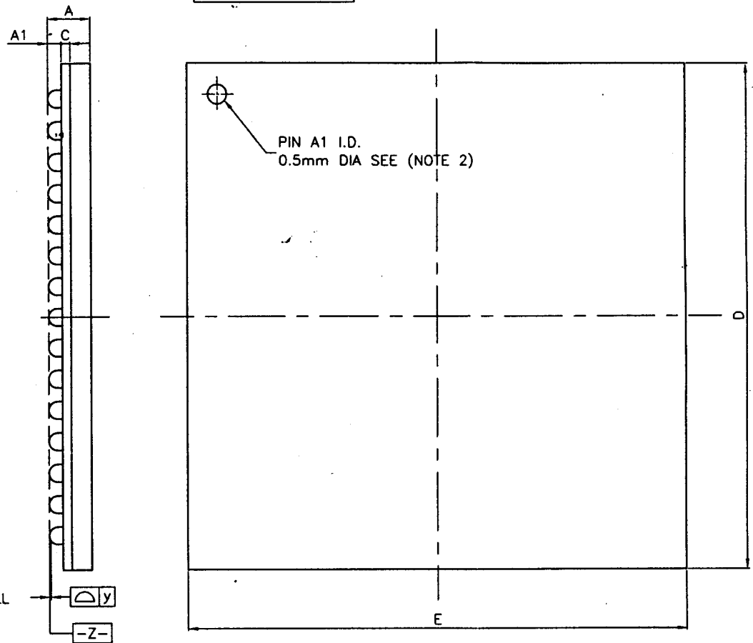
TOP SIDE TOP VIEW
