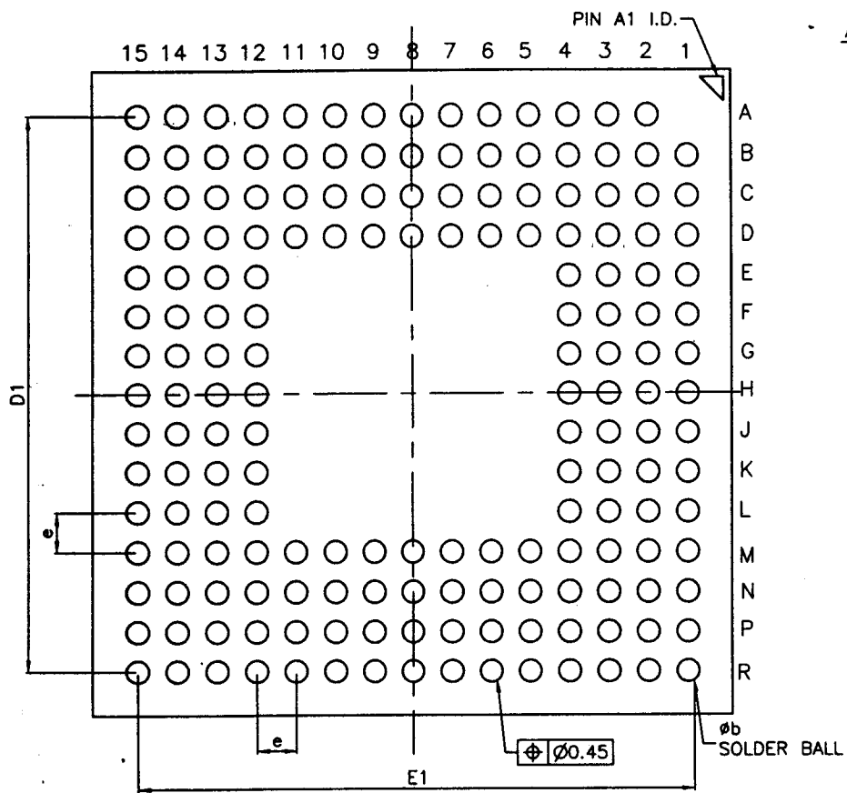
BOTTOM SIDE BOTTOM VIEW
