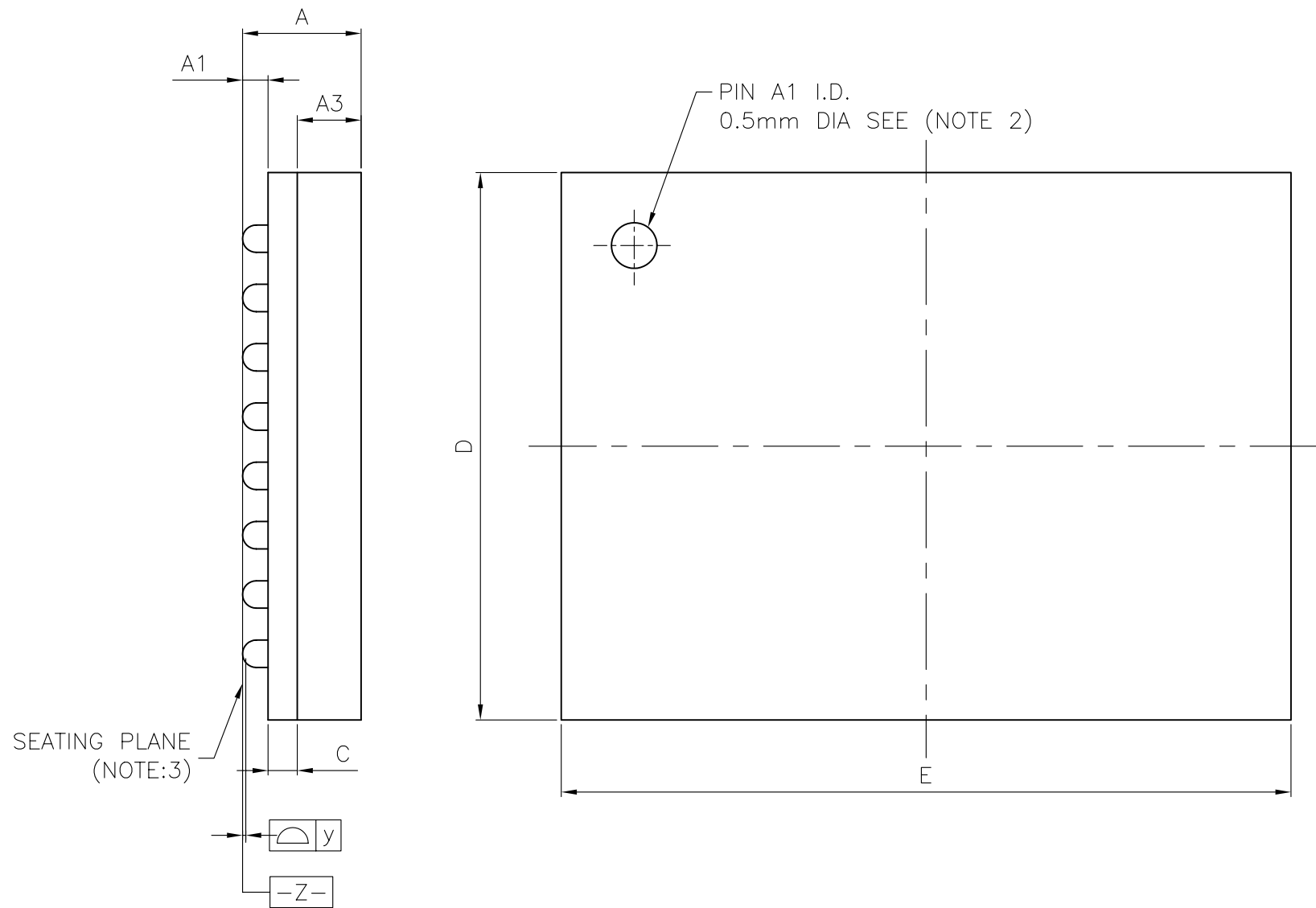
TOP SIDE TOP VIEW
