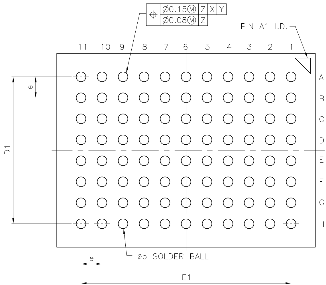
BOTTOM SIDE BOTTOM VIEW
