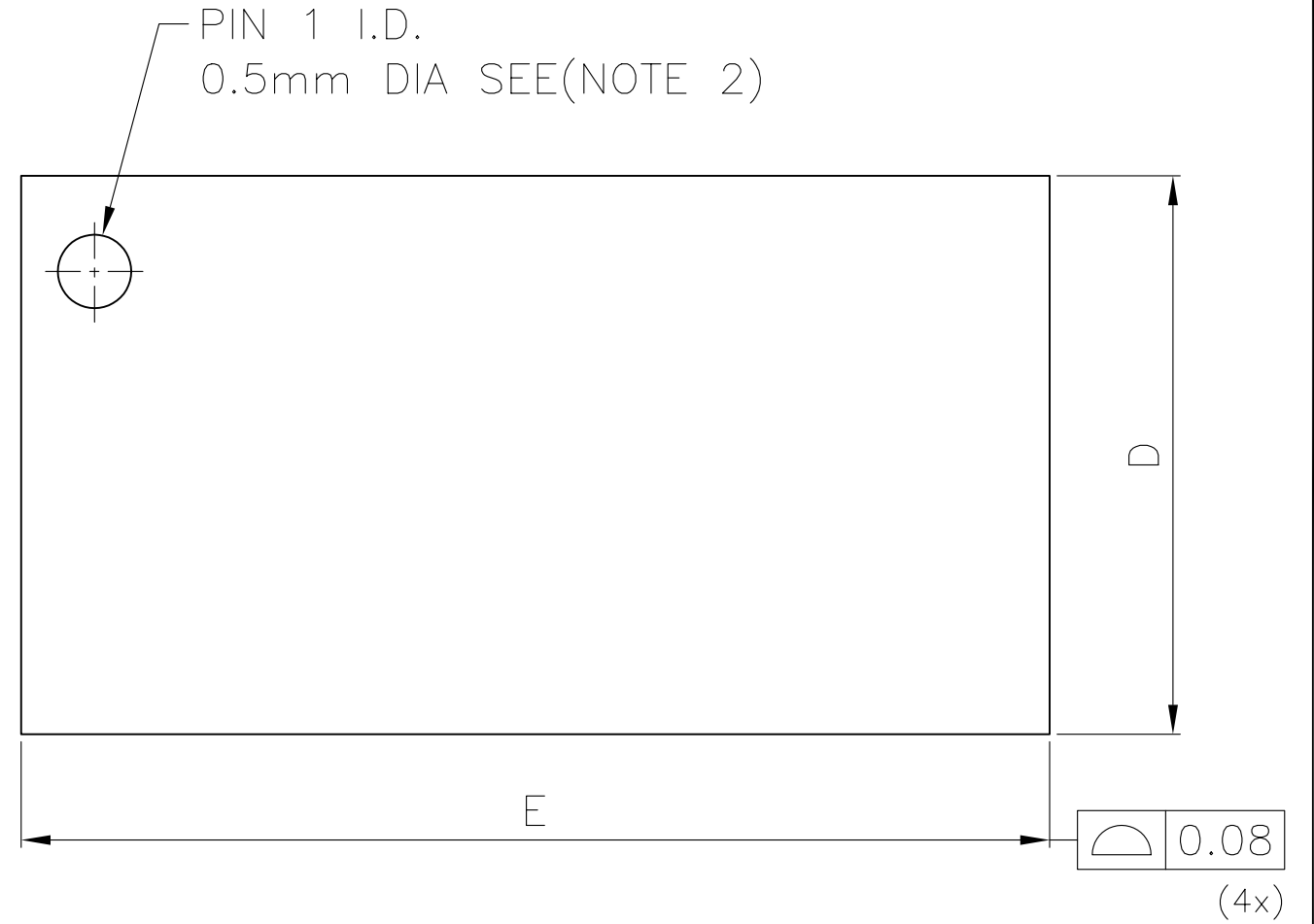
TOP VIEW
